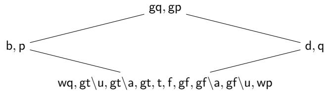
Fig. 2: Classes of consequence relations, from an abstract viewpoint
