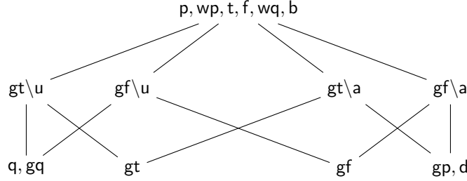
Fig. 1: Aspects of a given B-entailment relation
