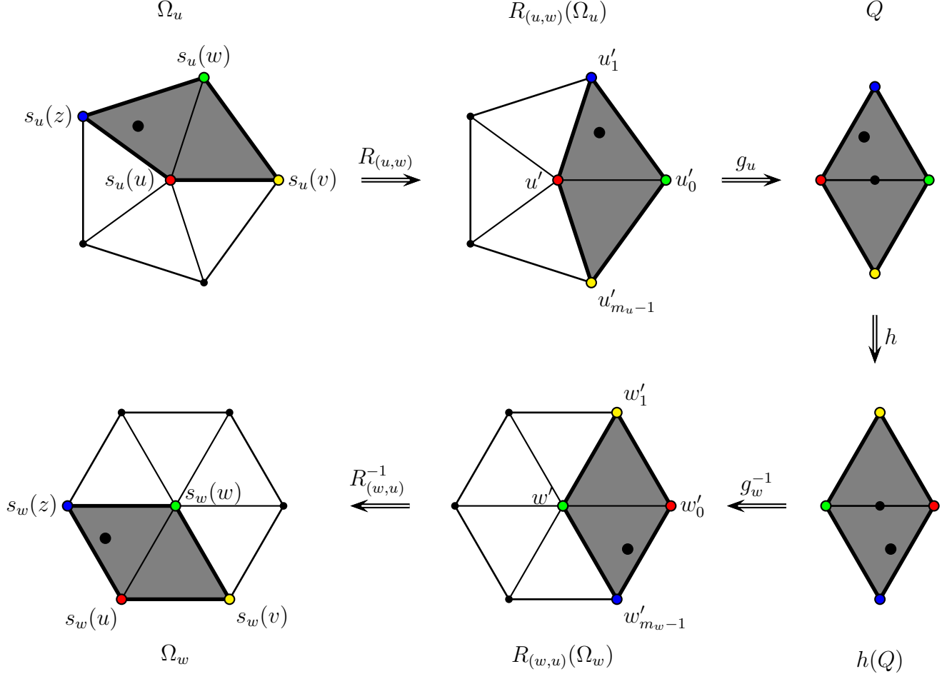
Figure 5.4: The transition function \varphi_{wu} .
