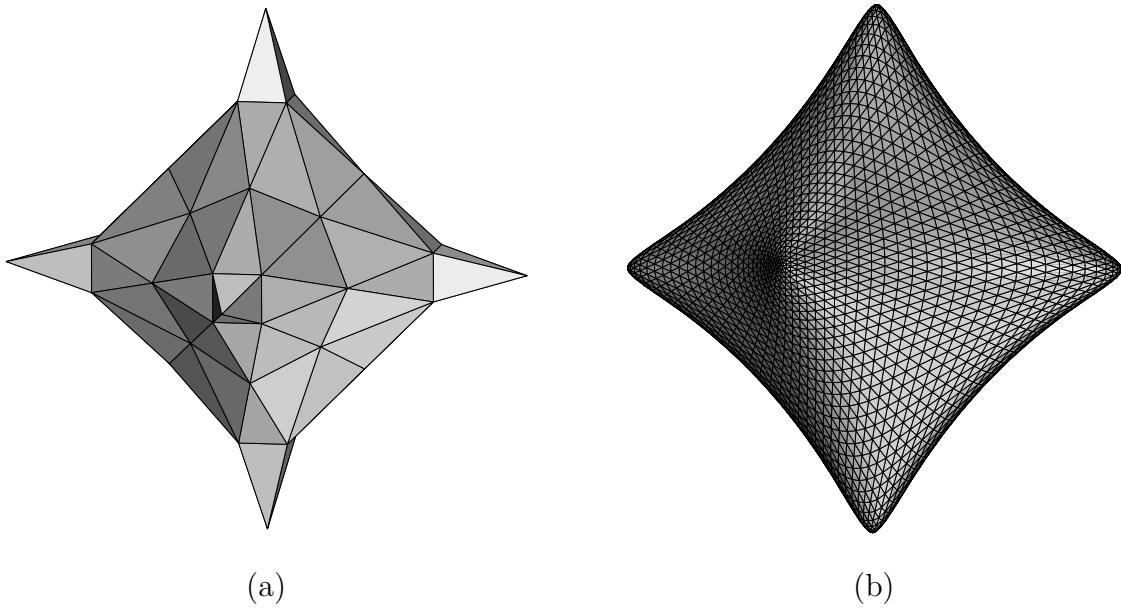
Figure 5.13: . (a) A star-shaped simplicial surface. (b) Approximation to a PPS defined from (a).
