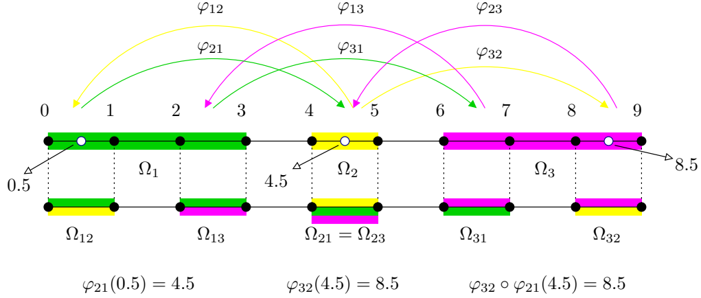
Figure 3.5: An example to show why condition (c') does not ensure the transitivity of \sim .
