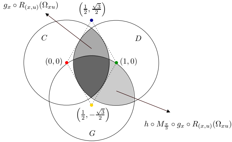
Figure A.2: The sets g_x \circ R_{(x,u)}(\Omega_{xu}) and h \circ M_{\frac{\pi}{3}} \circ g_x \circ R_{(x,u)}(\Omega_{xu}) .
