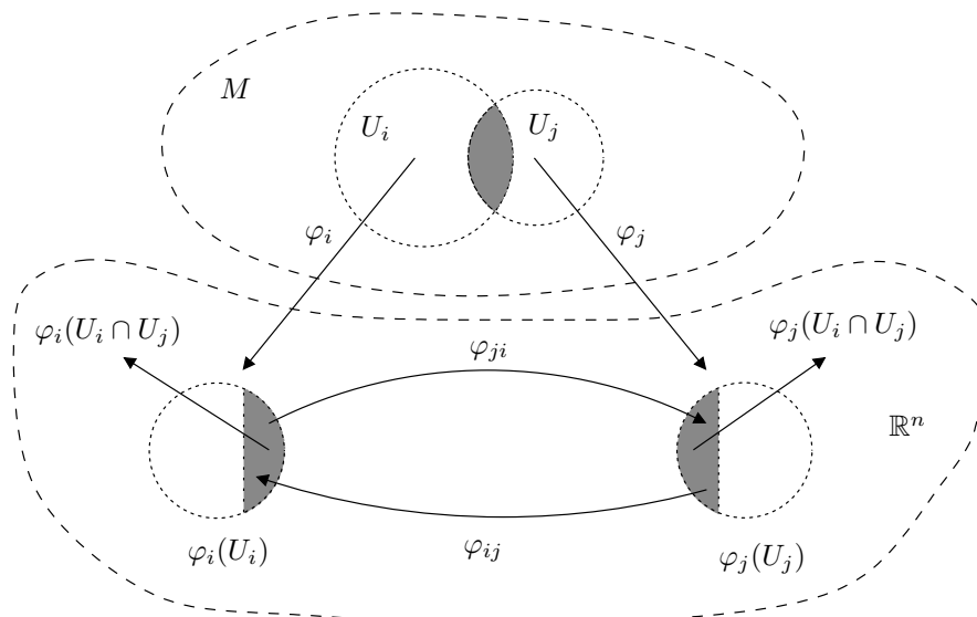
Figure 2.1: Illustration of the definition of transition maps.
