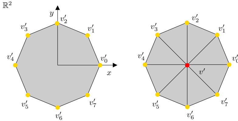
Figure 5.7: A P -polygon (left) and its canonical triangulation (right).
