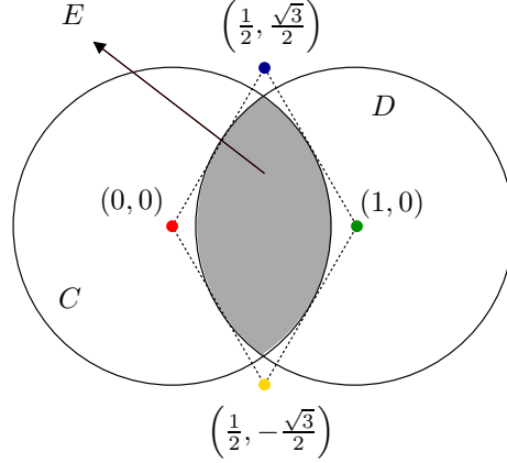
Figure 5.9: The circles C and D , the canonical lens E , and the quadrilateral Q (drawn with dotted line).
