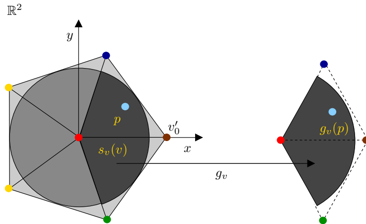
Figure 5.8: The action of g_v upon a point p \in C_v .
