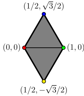
Figure 5.3: The canonical diamond Q .
