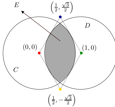
Figure 5.6: The circles C , D , and the canonical lens E .
