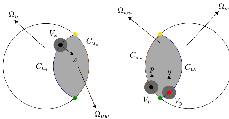
Figure A.5: The open balls V_x , V_y , and V_p .
