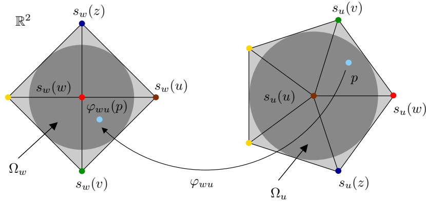
Figure 5.11: Illustration of Definition 5.9.
