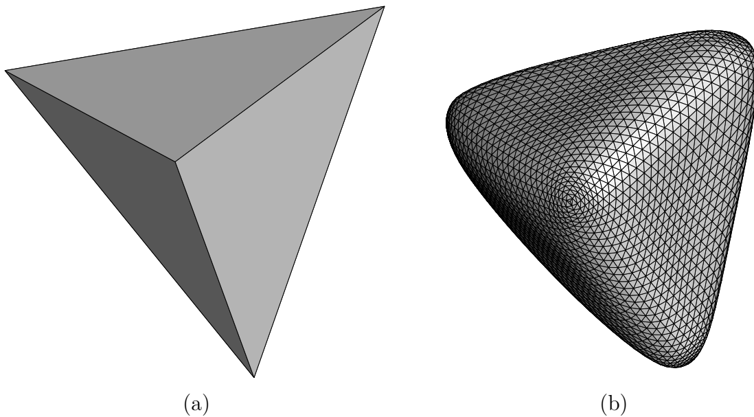
Figure 5.12: . (a) The boundary of a tetrahedron. (b) Approximation to a PPS defined from (a).
