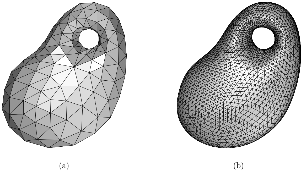
Figure 5.14: . (a) A simplicial surface. (b) Approximation to a PPS defined from (a).
