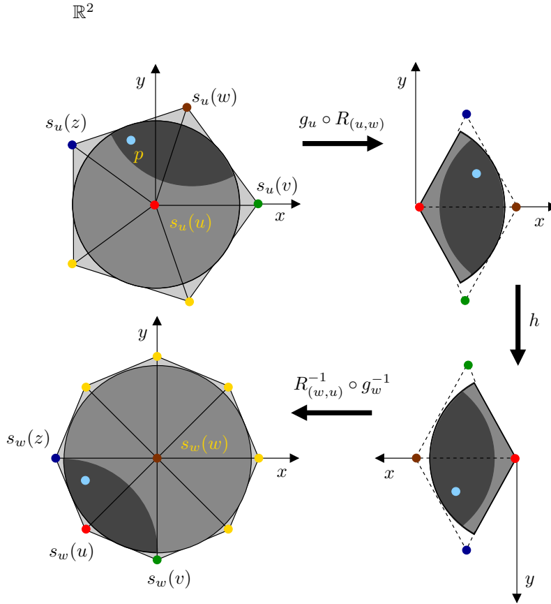
Figure 5.10: The action of g_{(u,w)} upon a point p \in G_{uw} , with G_{uw} = R_{(u,w)}^{-1} \circ g_u^{-1}(E) .
