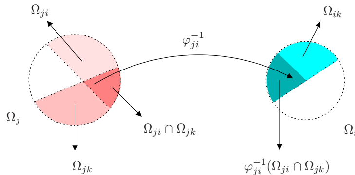
Figure 3.1: The cocycle condition of Definition 3.1.
