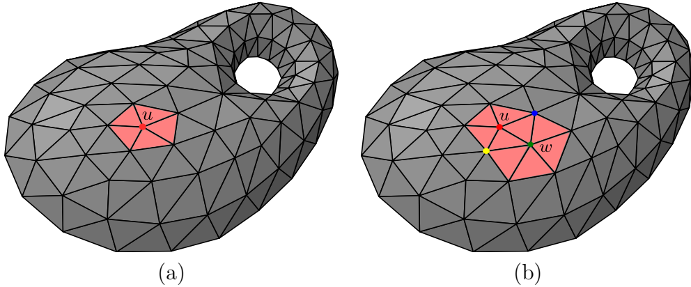
Figure 5.1: (a) The star of a vertex of a triangle mesh. (b) The stars of two adjacent vertices.
