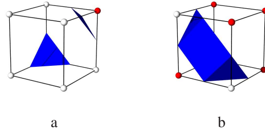
Fig. 15. The lookup table for the modified marching cubes algorithm has different reconstructions (a) and (b) for the complementary types of case 8.
