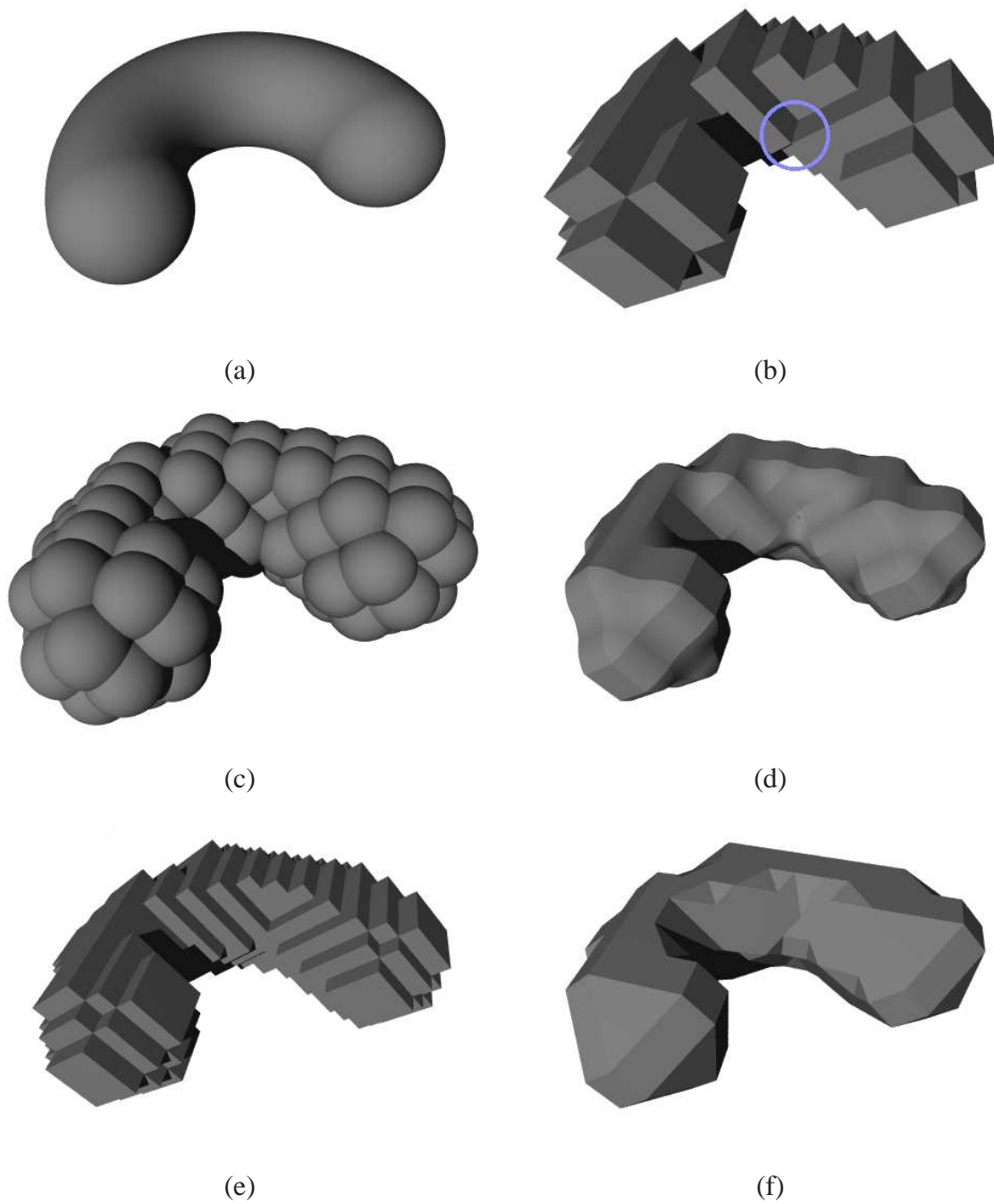
Fig. 19. Digitization of an r -regular object (a) with a cubic \frac{1}{2}r -grid. (b) digital reconstruction (Note that the surface is not a manifold inside the circle) (c) ball union, (d) trilinear interpolation, (e) majority interpolation and (f) modified marching cubes.
