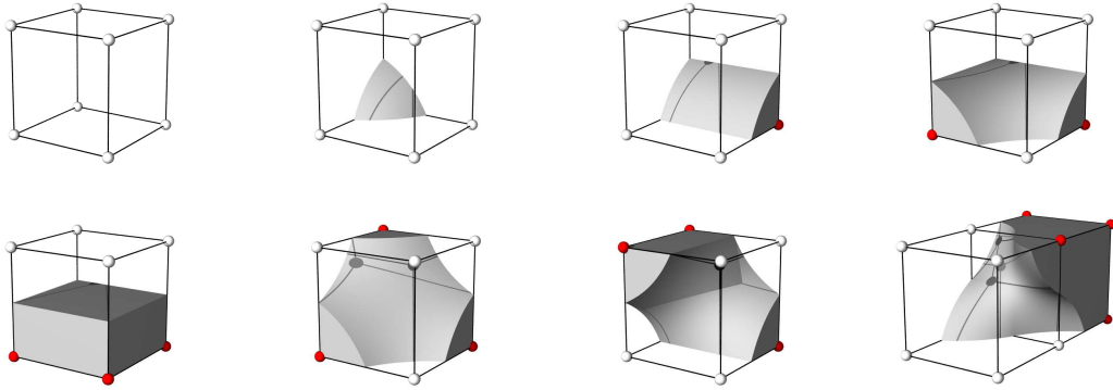
Fig. 16. Cases 1 to 8 for trilinear interpolation.
