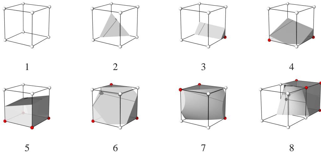
Fig. 9. The surface of the result of a topology preserving reconstruction method is homeomorphic to a disc inside any of the cubes of case 2 to 7 and the double-cube of case 8. The cube of case 1 does not intersect the surface.
