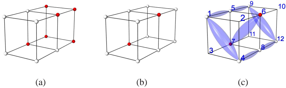
Fig. 8. Case 8 only occurs in complementary (a) and not in equal pairs (b).
