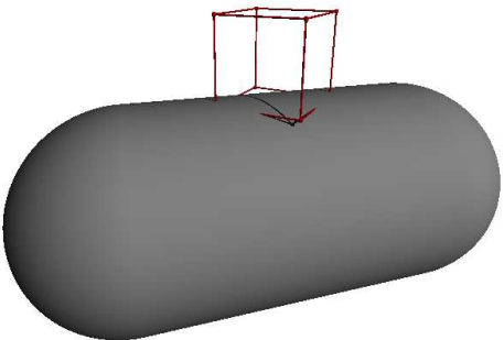
Fig. 4. The surface of an object only needs to have an arbitrarily small, but nonzero curvature in order to make occurrences of case 8 possible in the digital reconstruction.
