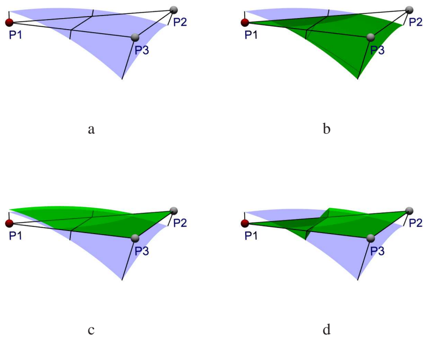
Fig. 12. In order to construct a surface between three sampling points being not all in the foreground (1), we combine the inner (2) and the outer surface patch (3) such that the result (4) is cut by \partial A into exactly two parts.
