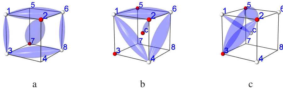
Fig. 7. Cases 9 to 14 are impossible in dense digitizations of r -regular objects.
