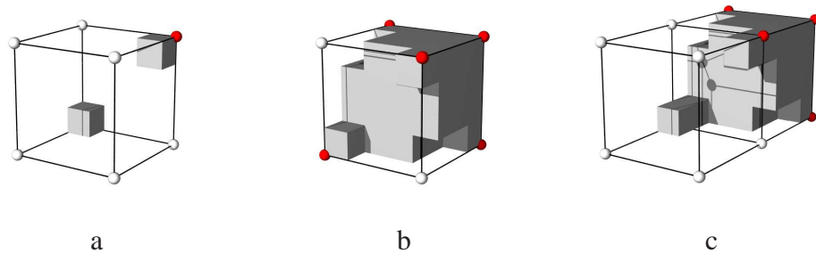
Fig. 11. The complementary occurrences (a) and (b) of case 8 can always be combined such that the surface inside the double cube is homeomorphic to a disc (c).
