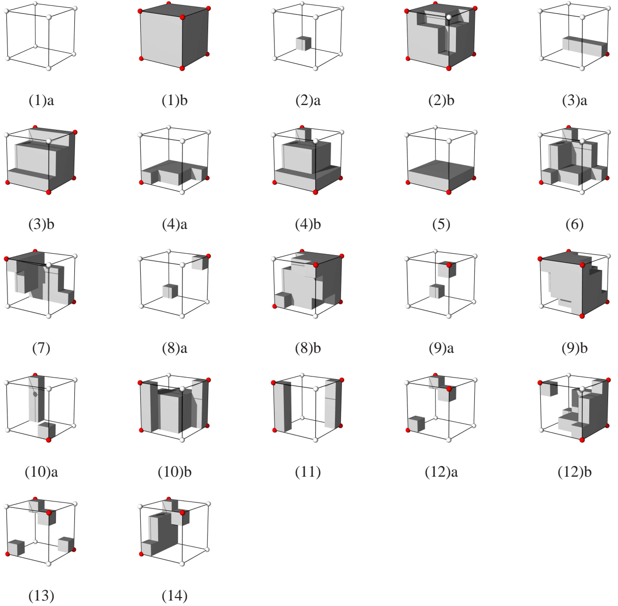
Fig. 10. The 22 different cases of Majority Interpolation (14 cases plus complementary cases).
