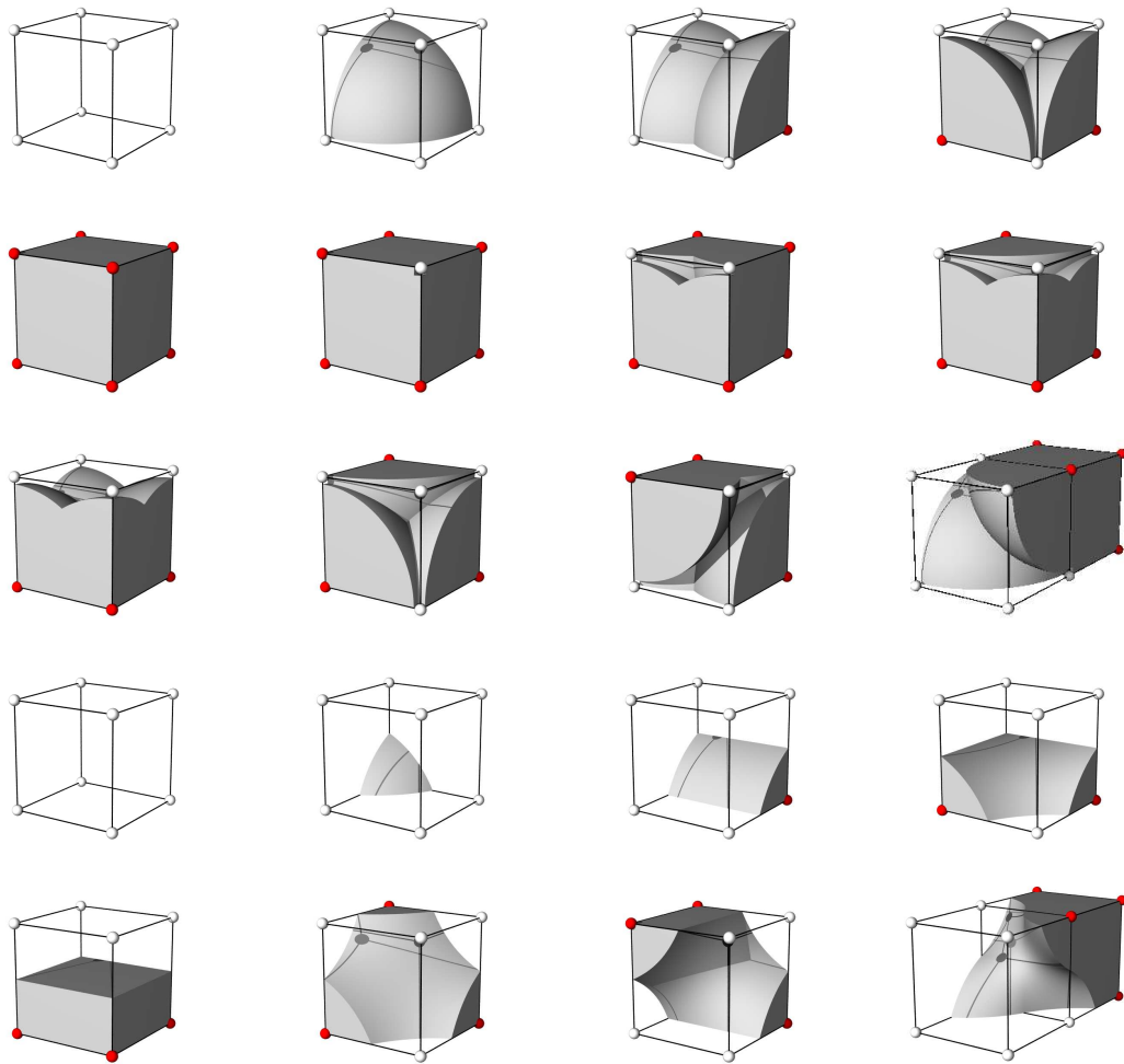
Fig. 13. First and second row: cases 1 to 4 for ball union and complementary subcases; third row: cases 5 to 8 for ball union.
