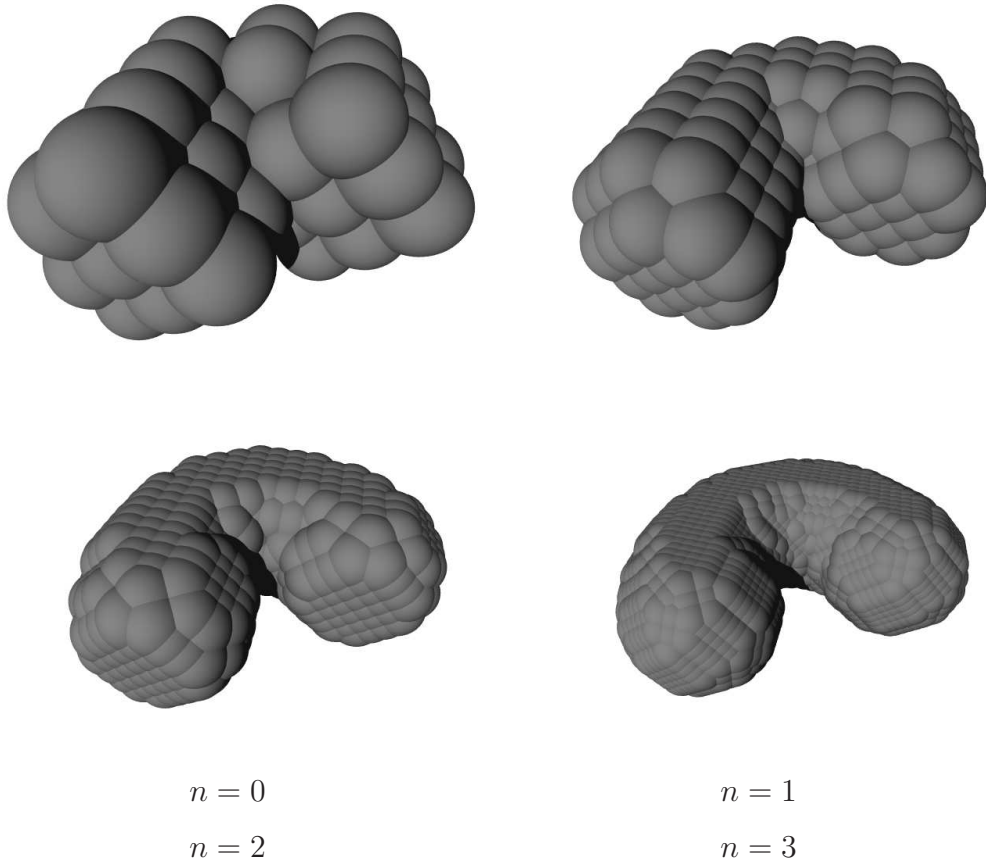
Fig. 20. C \oplus \mathcal{B}_s approximates \partial A with increasing n .
