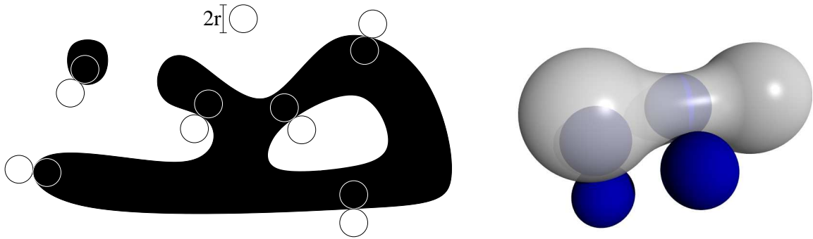
Fig. 1. For each boundary point of a 2D/3D r -regular set there exists an outside and an inside osculating open disc/ball of radius r .
