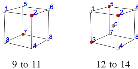
Fig. 6. Configurations 9 to 11 (resp. 12 to 14) in Fig. 5 can be summarized in special cases with “don’t care” sampling points p_4 and p_5 (resp. p_7 and p_8 ).
